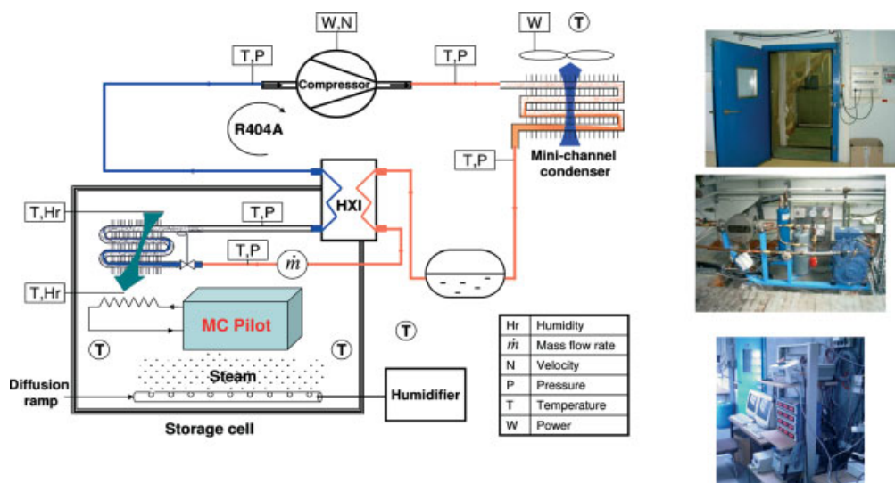
Figure 22.7 Layout of the system: membrane contactor and refrigerated cell of trucks or of storage cells.
