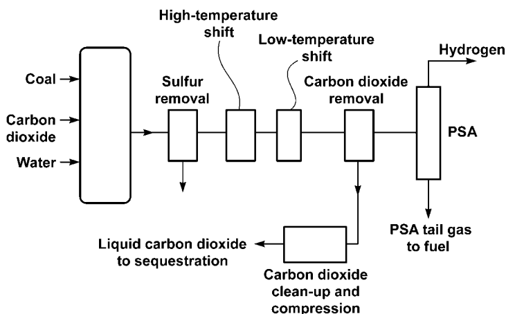
Figure 8.17 Block diagram of a coal-to-hydrogen production plant. Many variants of the process have been proposed.
