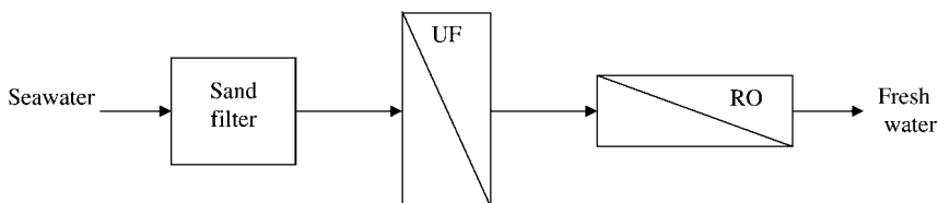
Figure 12.1 Scheme of an UF-RO membrane integrated desalination system [8].
