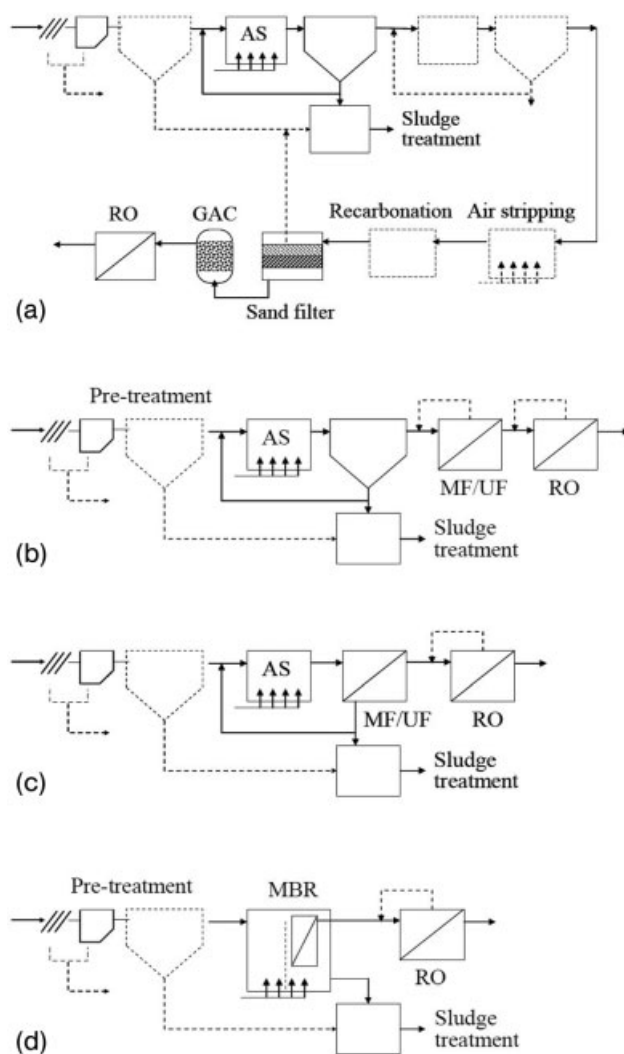
Figure 16.1 Illustration of evolution and use of membranes in wastewater treatment.
