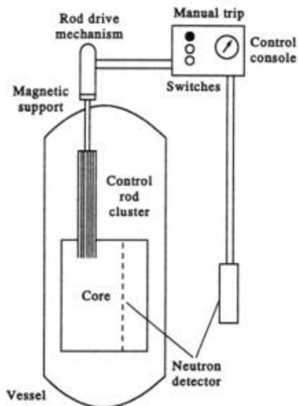
FIG. 19.4 Reactor control.
