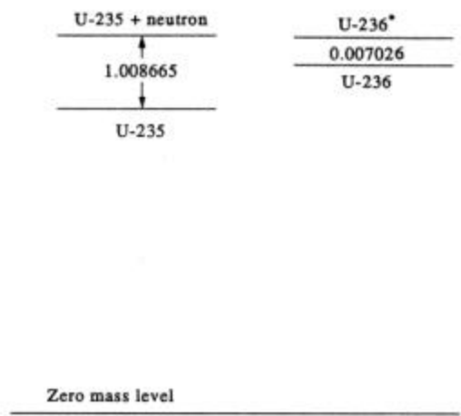
FIG. 6.2 Excitation energy due to neutron absorption.
