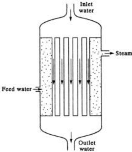
FIG. 12.6 Heat exchanger or steam generator.
