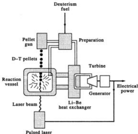
FIG. 14.6 Laser-fusion reactor.
