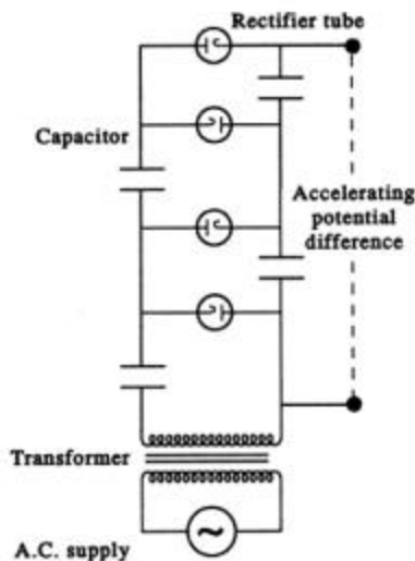
FIG. 8.4 Cockroft-Walton circuit.
