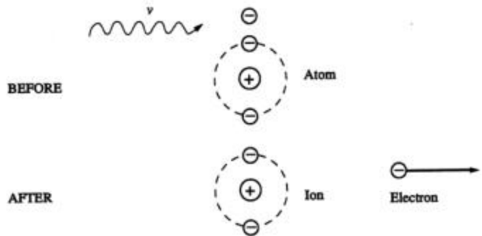
FIG. 5.5 Photoelectric effect.
