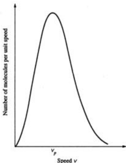
FIG. 2.1 Distribution of molecular speeds.
