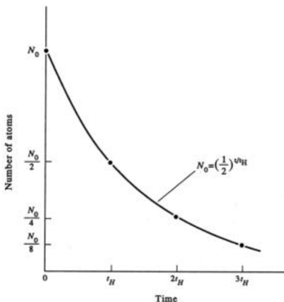
FIG. 3.1 Radioactive decay.
