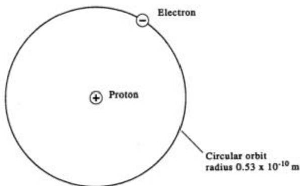
FIG. 2.2 Hydrogen atom.
