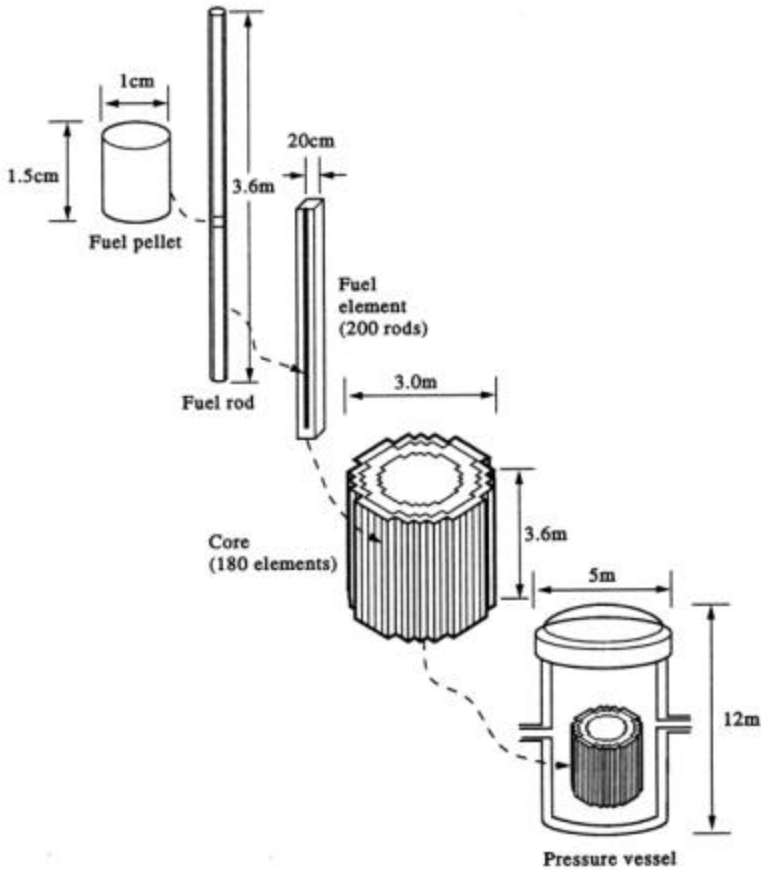
FIG. 11.5 Reactor construction.
