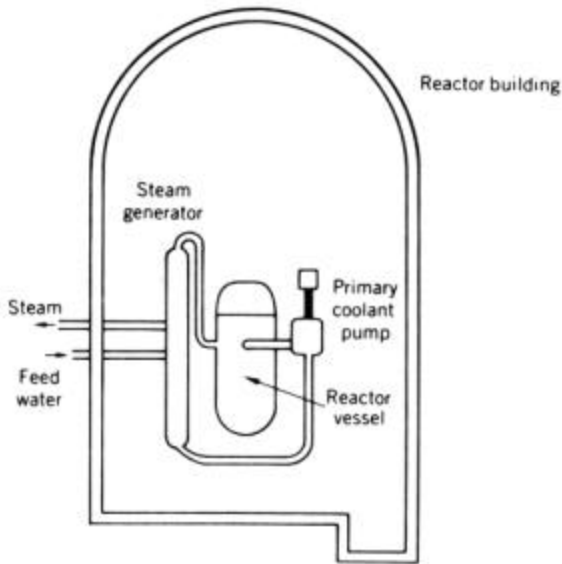
FIG. 19.8 Reactor containment.
