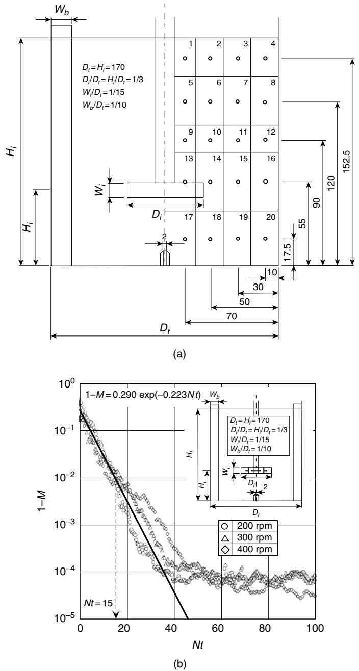
Figure 2.8 (a) Aerated stirred vessel and imaginary partition of vessel. (b) Relationship between mixedness and dimensionless time in an aerated stirred vessel.
