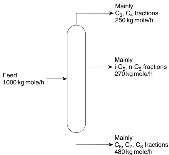
Figure 3.4 Distillation column.
