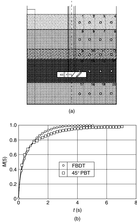
Figure 2.16 (a) Initial setting of five components in a stirred vessel. (b) Mixedness change with time of five-component mixing in case of FBDT impeller and 45° PBT impeller in a stirred vessel.
