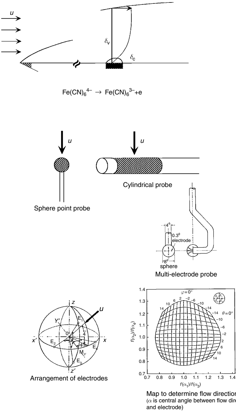
Figure 4.13 Velocity-measuring probes based on electrode reaction controlled by mass transfer rate.
