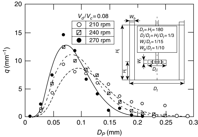
Figure 5.2 Data of droplet size probability density distribution in liquid-liquid mixing and fitted PSD curve based on new PSD function.
