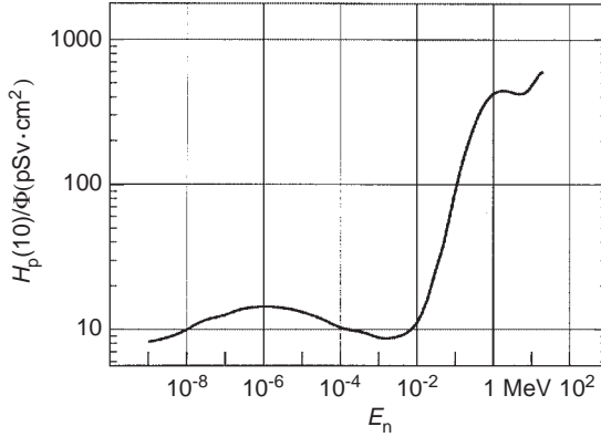
FIG. 28. Variation of quotient H_p(10)/\Phi with energy E_n of monodirectional and monoenergetic neutron radiation.
