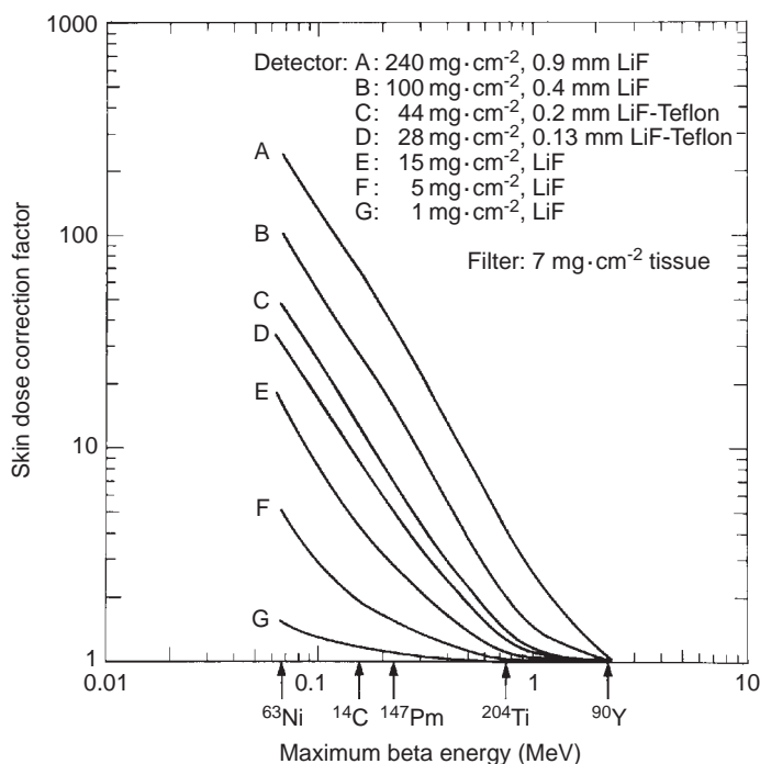
FIG. 24. Dependence of skin dose correction factor on maximum beta ray energy for different LiF detector thicknesses [53].
