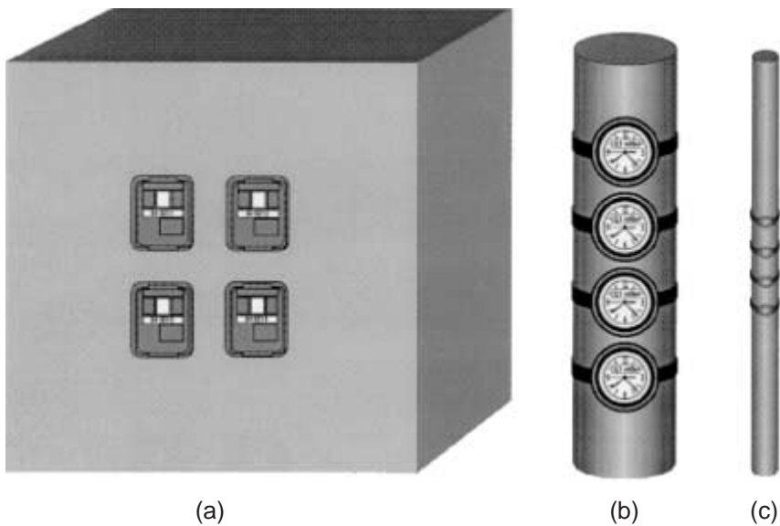
FIG. 4. Phantoms for calibrating personal dosimeters. (a) ISO water slab phantom, (b) ISO water pillar phantom, (c) ISO PMMA rod phantom. As an example, four dosimeters are attached to each phantom [9].
