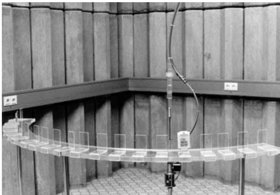
FIG. 19. Uncollimated gamma irradiation system.
