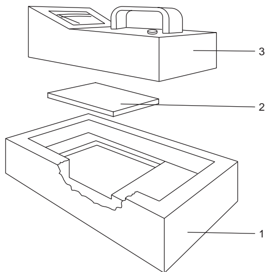
FIG. 35. Calibration set-up for surface contamination meters. (1) Source holder for standard geometry; (2) reference standard source; (3) instrument.
