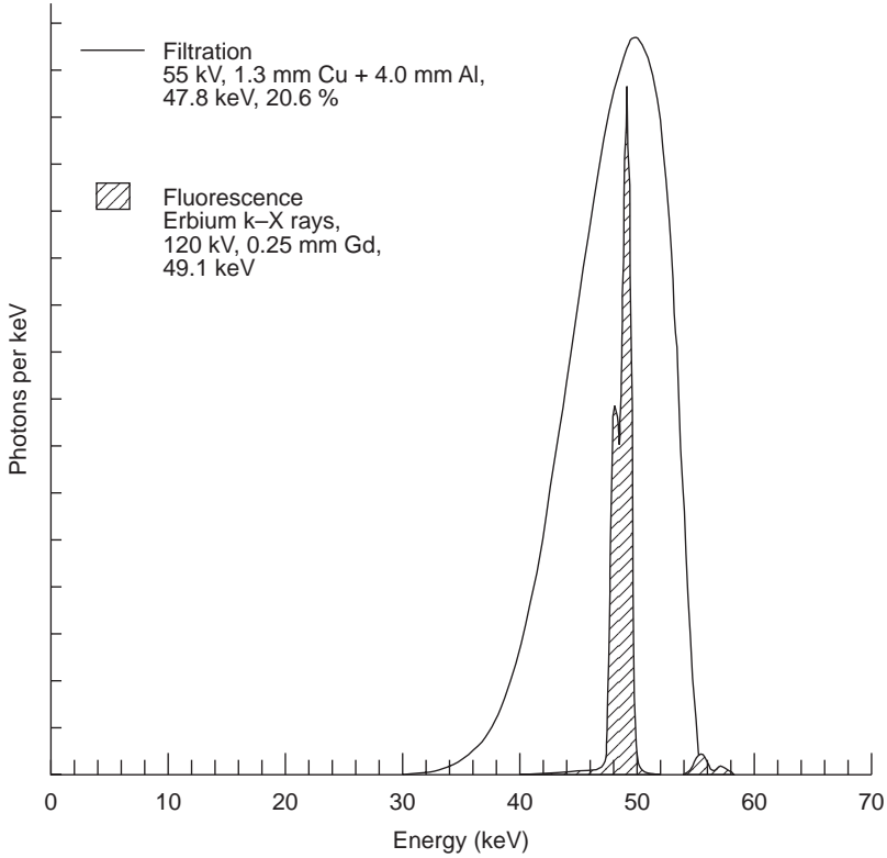
FIG. 8. Comparison of spectra of ISO low air kerma rate filtered reference radiation and ISO fluorescence reference radiation.
