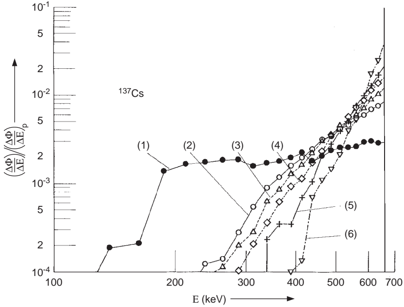
FIG. 13. Spectral photon fluence distributions for beam without absorber (1), and for beam with lead absorbers of different thicknesses, (2)–(6) [0.693, 1.100, 1.609, 2.203 and 4.605 cm]. \Delta\phi/\Delta E is the spectral fluence (quotient of the fluence \Delta\phi and the energy interval \Delta E ; \Delta E = 5 keV) and (\Delta\phi/\Delta E)_p is the spectral fluence of the primary photons [34].
