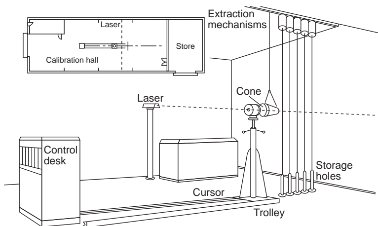
FIG. 30. Layout of calibration facility.
