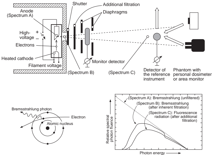
FIG. 9. X ray radiation measurement.
