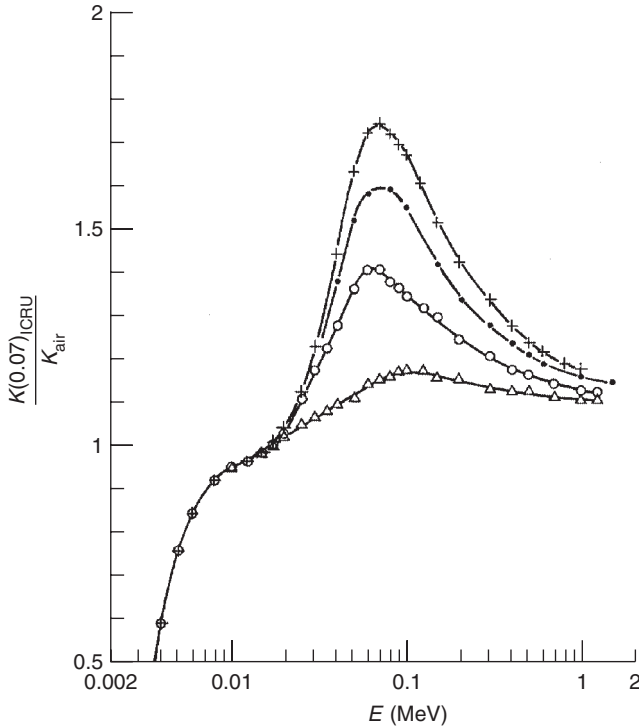
FIG. 7. Ratio of ICRU tissue kerma in the slab (+), pillar (•), rod (o) and sphere (Δ) phantoms of ICRU tissue at a depth of 0.07 mm and the air kerma free in air as a function of photon energy [10].
