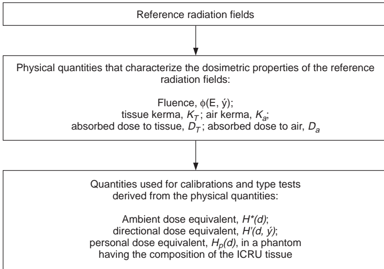
FIG. 1. Reference radiation fields, physical quantities that characterize the dosimetric properties of the reference radiation fields, and quantities used for calibrations and type tests.
