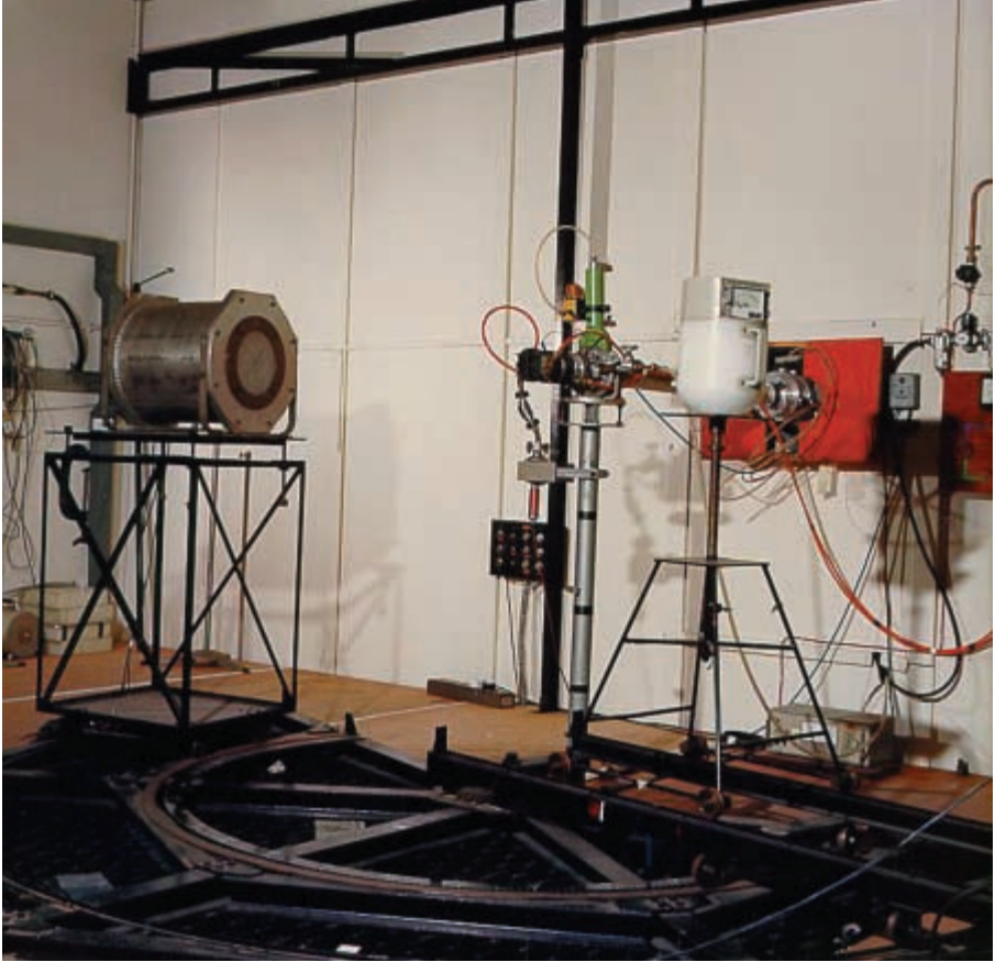
FIG. 31. Support system for neutron reference instrument (precision long counter) and for neutron measuring instrument (rem counter) used during calibration with a neutron generator (accelerator).
