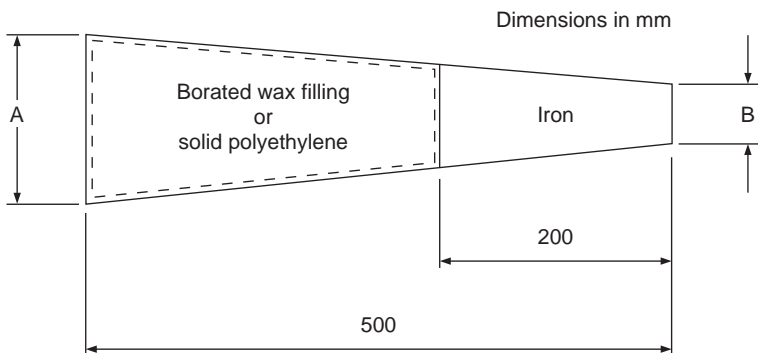
FIG. 32. Dimensions and construction of shadow cone.
