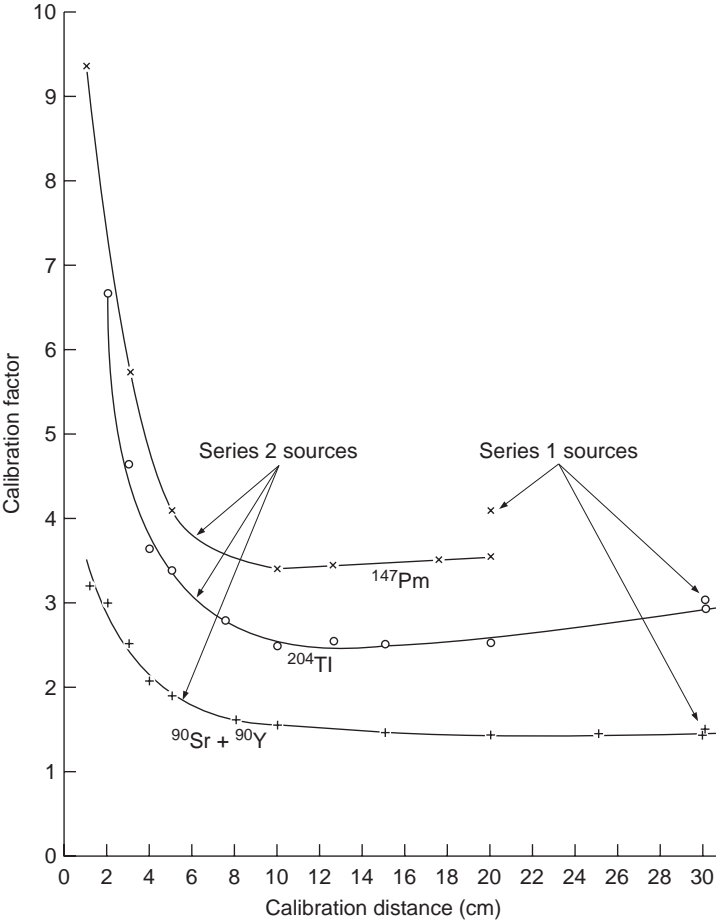
FIG. 26. Calibration factors of a portable dose rate instrument with a thin walled ionization chamber as a function of calibration distance for Series 1 and 2 sources. The reference point has been taken to be the entrance window.
