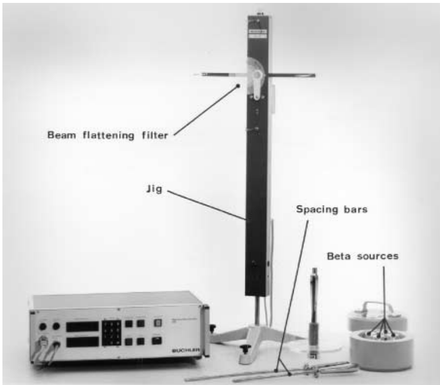
FIG. 27. Calibration stand for Series 1 and 2 reference beta radiations [41]. Left: control unit for the remote control of the shutter with digital preselection of its opening time; middle: jig for the beta ray source support with the shutter and beam flattening filter; right: container for storing the four beta sources; spacing bars and handling tool for manipulating the beta ray sources.
