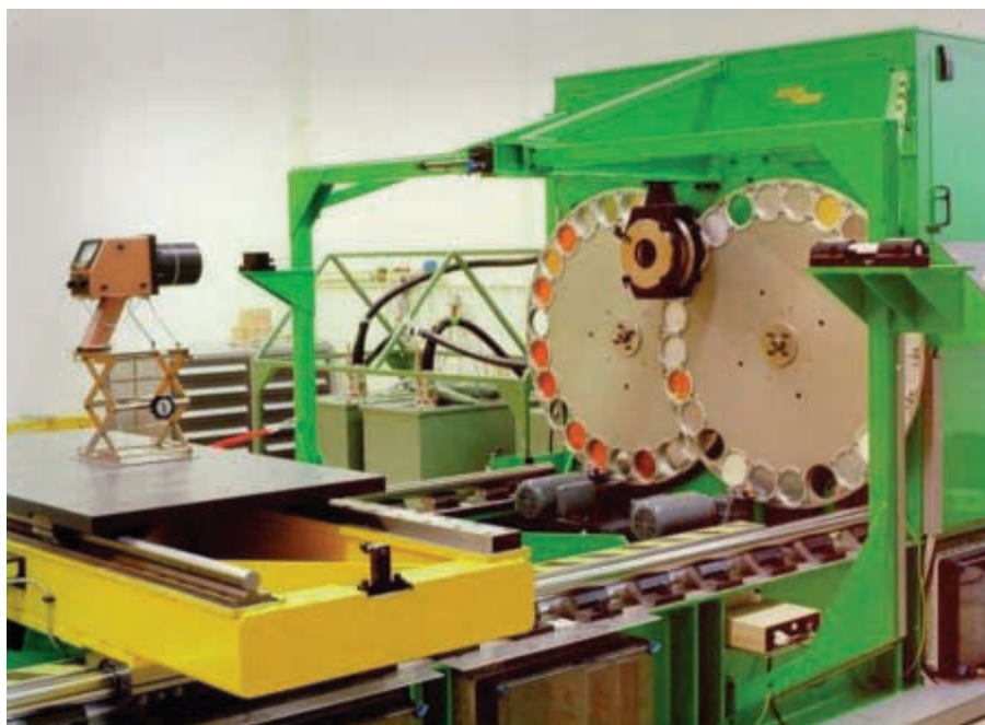
FIG. 20. Computer controlled combined X ray filtered and fluorescent irradiation system.
