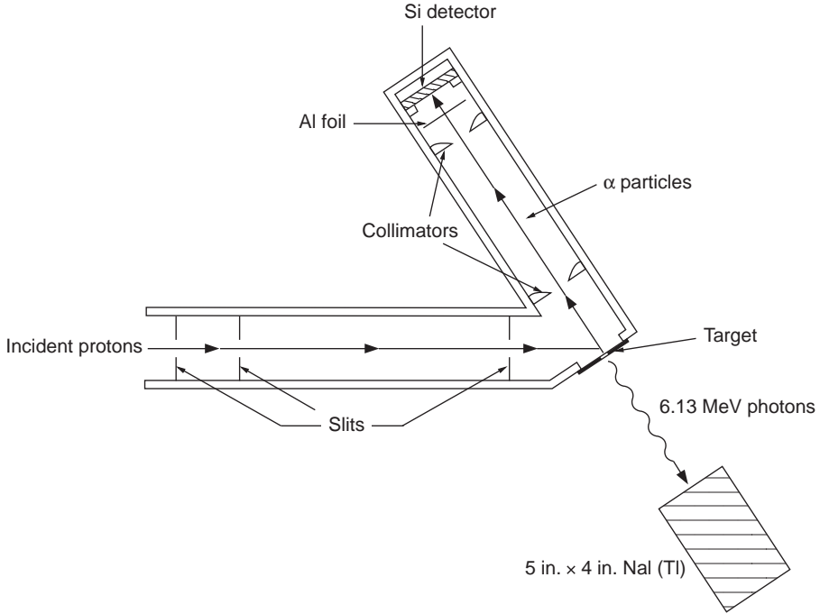
FIG. 14. Counting set-up for alpha particle measurements.
