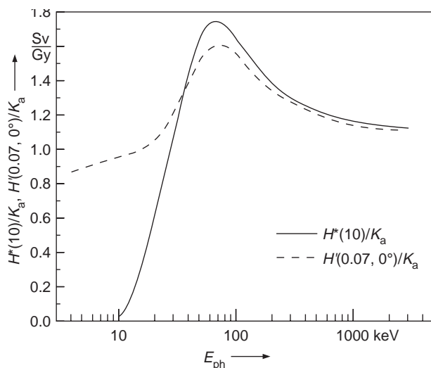
FIG. 6. Conversion coefficient H from air kerma K_\alpha to H^*(10) and to H'(0.07, 0^\circ) for monoenergetic photon radiation of energy E_{ph} .
