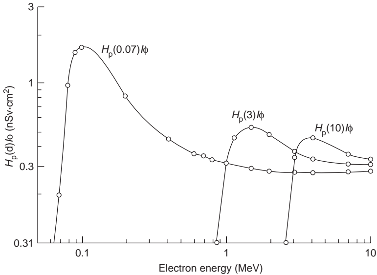
FIG. 21. Conversion coefficients relating personal dose equivalent in the slab phantom (depths: 0.07, 3 and 10 mm) to fluence for monoenergetic electrons impinging on the slab phantom at normal incidence.
