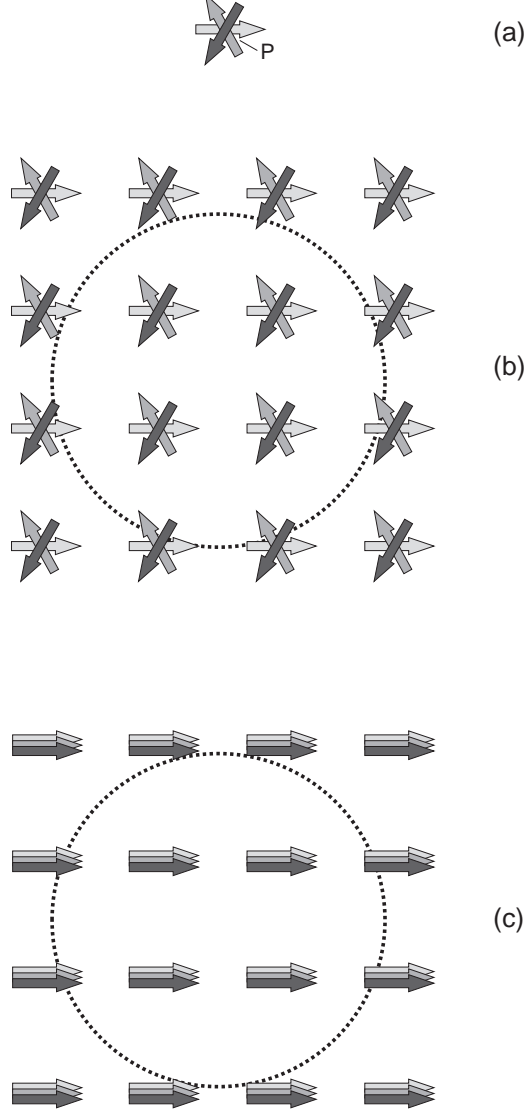
FIG. 2. Schematic representation of (a) a real radiation field, (b) an expanded radiation field, and (c) an expanded and aligned radiation field [9]. (a) Actual radiation field at the point of interest, P, consisting of three components of different directions, symbolized by three different arrows. (b) Expanded radiation field belonging to point P. The dotted circle is drawn to illustrate the required size for the expanded field. (c) Expanded and aligned field belonging to point P. The circle is drawn to illustrate the required size for the expanded and aligned field. In principle, the three arrows at each location are strictly coincident, but for reasons of clarity are shown in succession.
