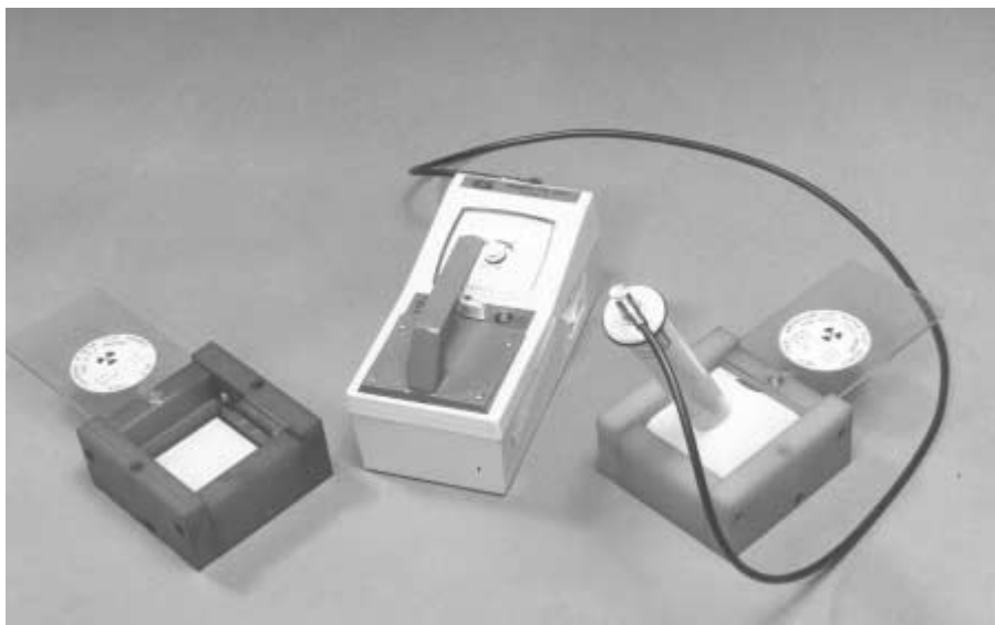
FIG. 34. Set of reference standard sources for calibration of surface contamination meters and monitors.
