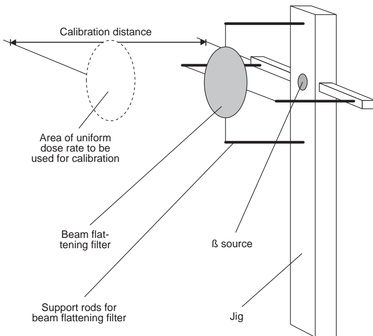
FIG. 22. Calibration stand with beam flattening filter.
