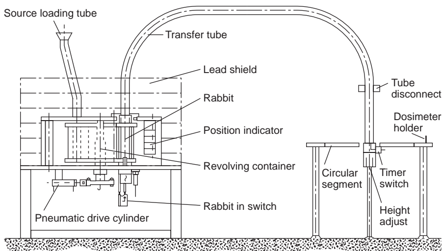
FIG. 18. Schematic design of an example of an uncollimated irradiation system [37].
