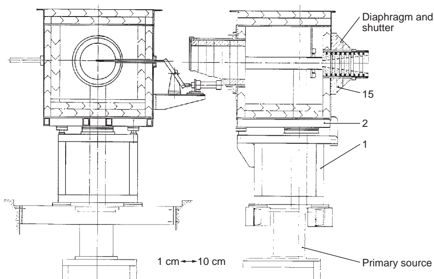
FIG. 12. Example of a collimated irradiation system with conical ring collimator.
