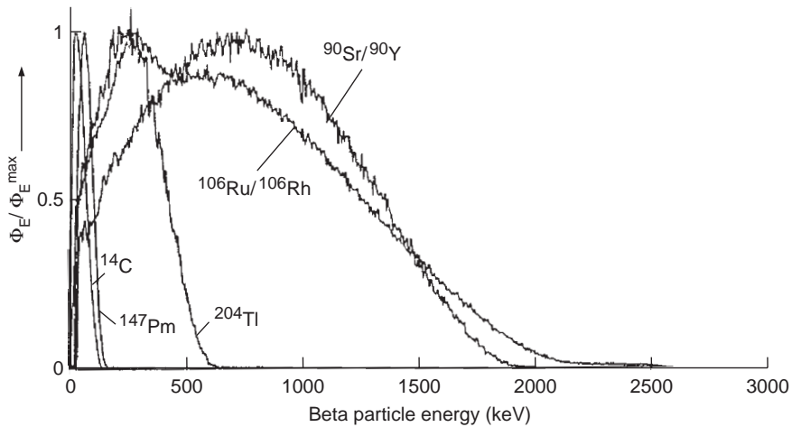
FIG. 25. Examples of beta particle spectra for Series 1 and 2 reference beta radiations measured at the calibration distances with effectively windowless uncooled Si(Li) semiconductor detectors. The measured flux densities \Phi_E are normalized to the same maximum value \Phi_E^{\text{max}} , but not corrected for instrumental resolution or detector backscattering loss.
