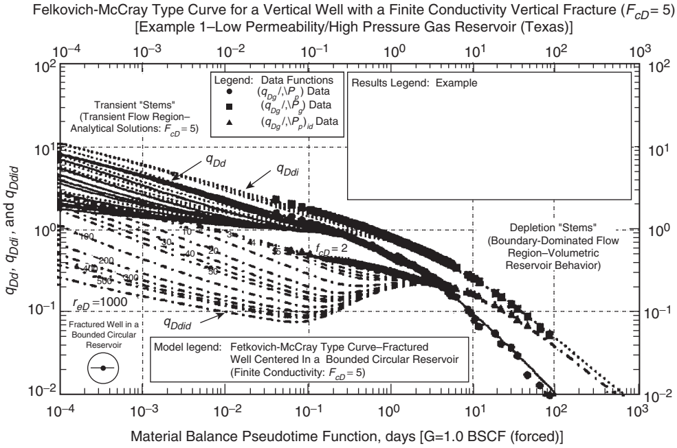
Figure 3.72 Match of production data for Example 1 on the Felkovich-McCray decline type curve (pseudopressure drop normalized rate versus material balance time format) for a well with a finite conductivity vertical fracture ( F_{CD} = 5 ) (Permission to copy by the SPE, 2003).
