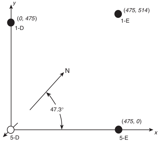
Figure 1.106 Well locations for Example 1.43 (After Earlougher, R. Advances in Well Test Analysis ) (Permission to publish by the SPE, copyright SPE, 1977).
