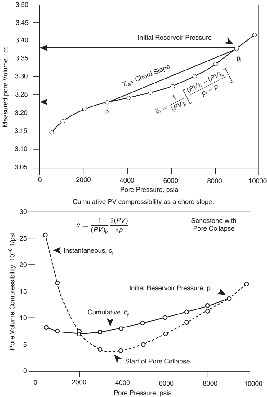
Figure 3.27 Cumulative and instantaneous c_i .
