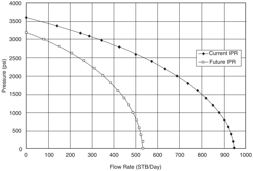
Figure 5.22 IPR.
