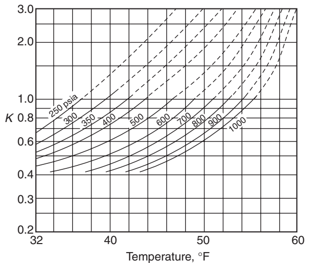
Figure 3.86 Vapor–solid equilibrium constant for \text{CO}_2 (Carson & Katz, 1942, courtesy SPE-AIME).
