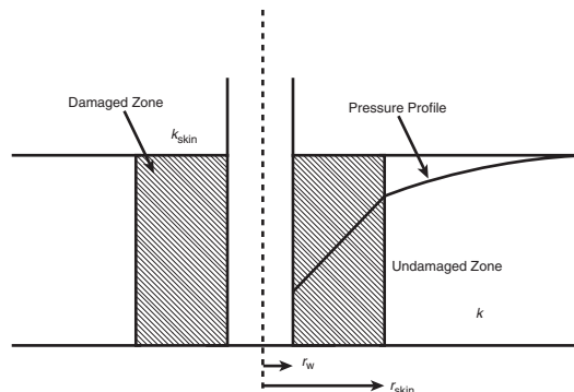
Figure 1.26 Near-wellbore skin effect.
