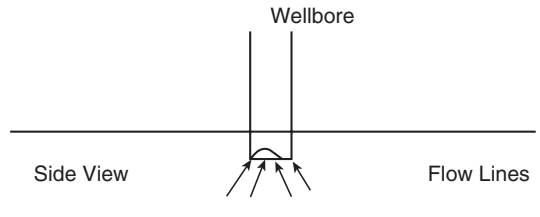
Figure 1.8 Hemispherical flow in a partially penetrating well.
