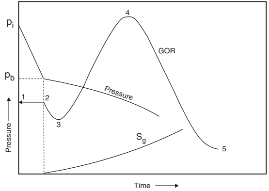
Figure 5.1 Characteristics of solution gas drive reservoirs.
