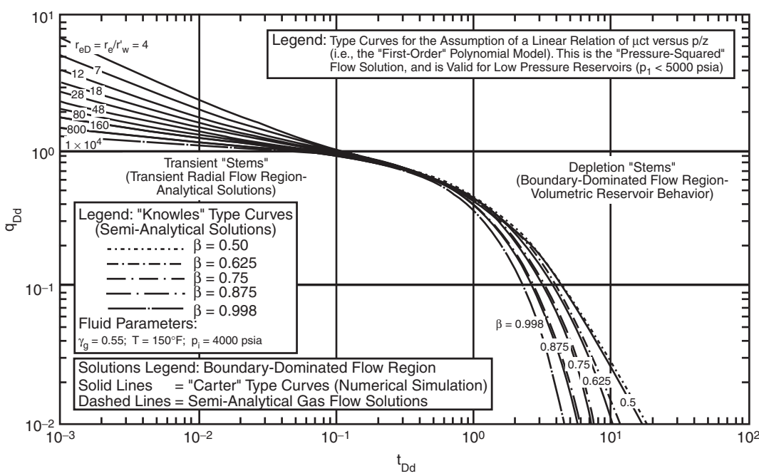
Figure 3.63 “First-order” polynomial solution for real-gas flow under boundary-dominated flow conditions. Solution assumes a \mu c_i profile that is linear with p_D (Permission to copy by the SPE, 2000).
