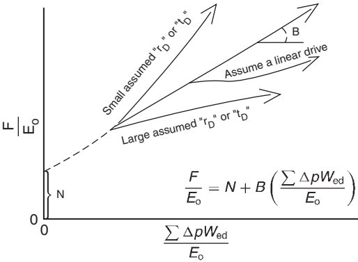
Figure 4.27 Havlena and Odeh straight-line plot (After: Havlena and Odeh, 1963).
