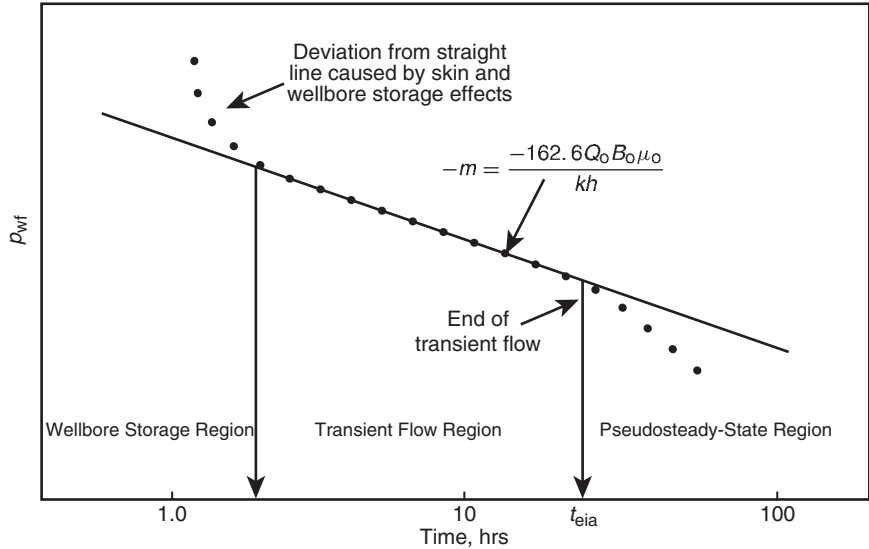
Figure 1.33 Semilog plot of pressure drawdown data.
