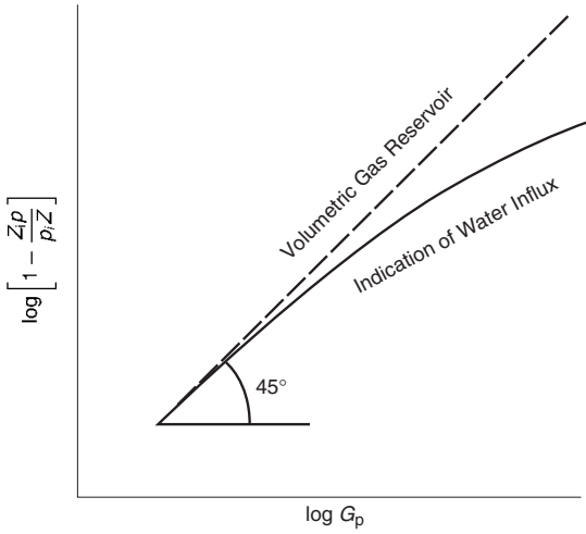
Figure 3.21 Energy plot.
