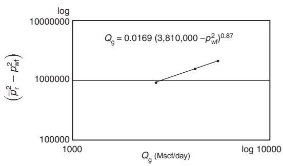
Figure 3.9 Back-pressure curve.
