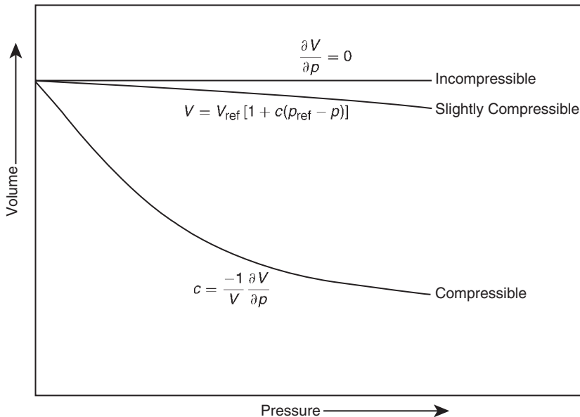
Figure 1.1 Pressure–volume relationship.
