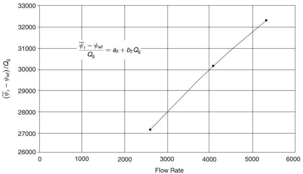
Figure 3.12 Pseudopressure method.
