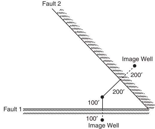
Figure 1.31 Well layout for Example 1.23.
