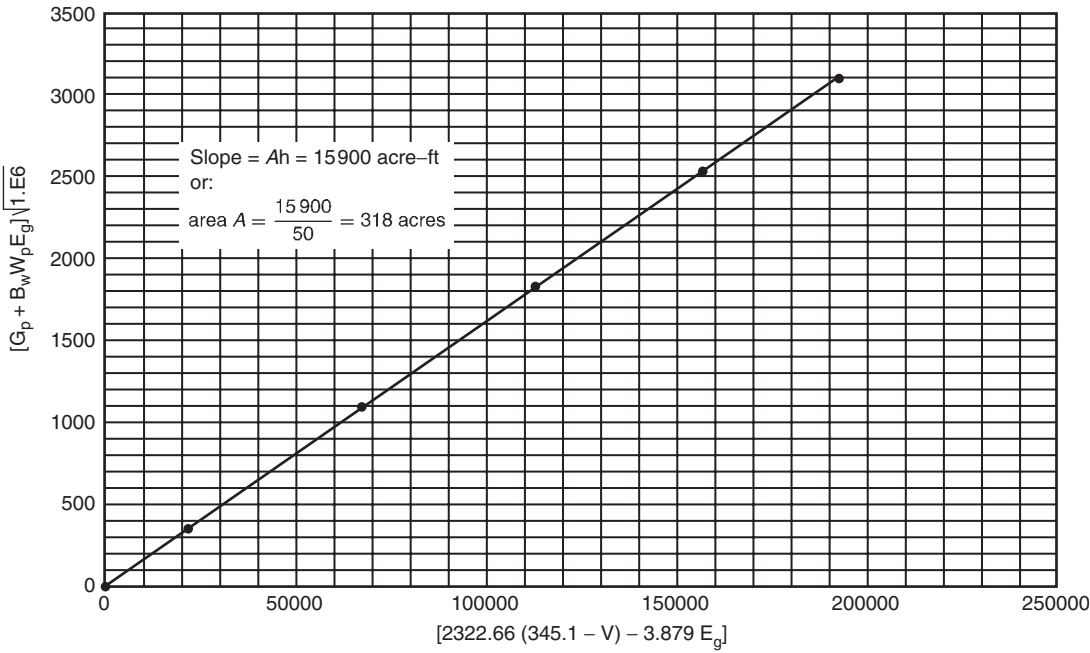
Figure 3.37 Graphical determination of drainage area.
