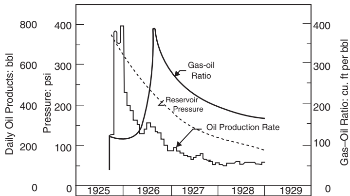
Figure 4.2 Production data for a solution gas drive reservoir. (After Clark, N.J., Elements of Petroleum Reservoirs , SPE, 1969).
