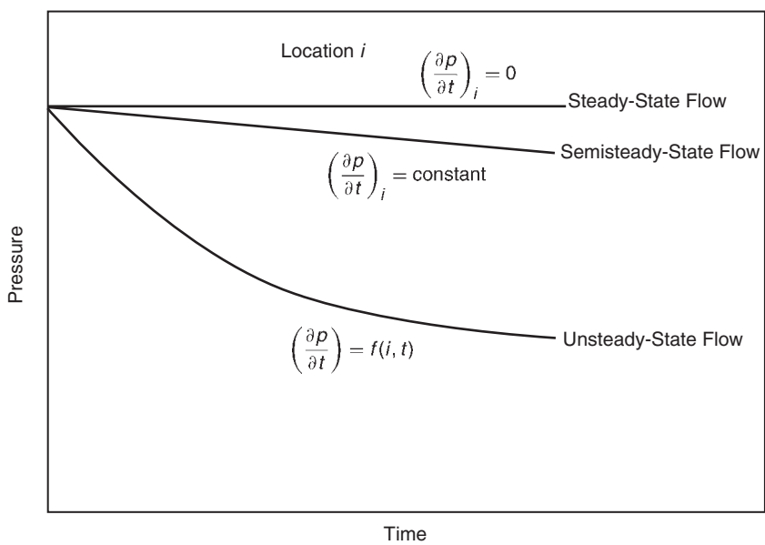
Figure 1.3 Flow regimes.
