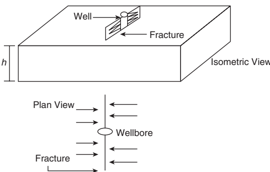
Figure 1.6 Ideal linear flow into vertical fracture.
