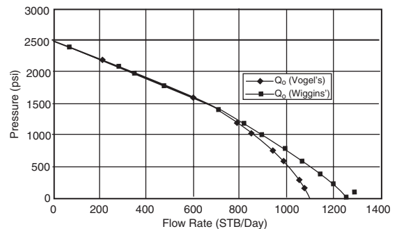
Figure 5.17 IPR curves.
