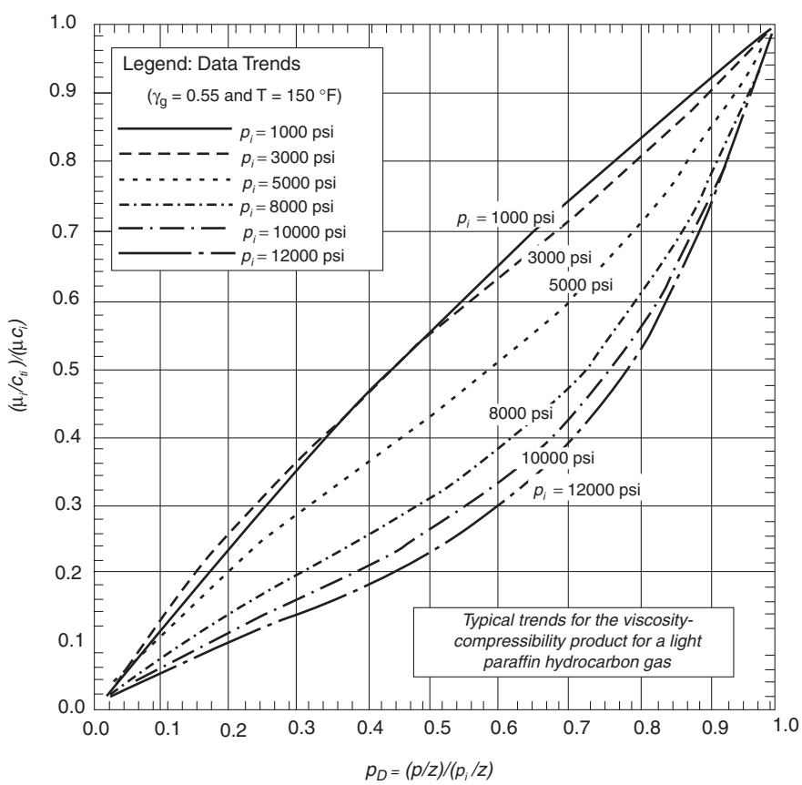
Figure 3.62 Typical distribution of the viscosity–compressibility function (After Anash et al., 2000).
