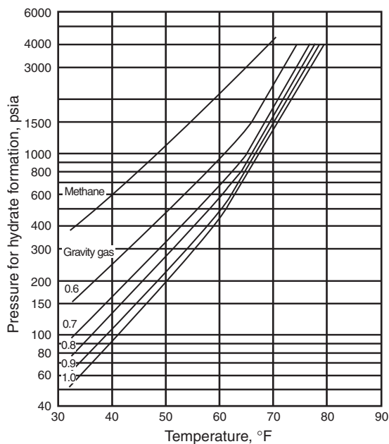
Figure 3.74 Pressure-temperature curves for predicting hydrate (Courtesy Gas Processors Suppliers Association).
