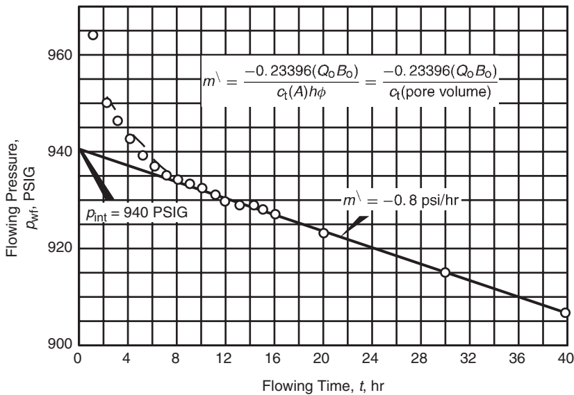
Figure 1.35 Cartesian plot of the drawdown test data (Permission to publish by the SPE, copyright SPE, 1977).
