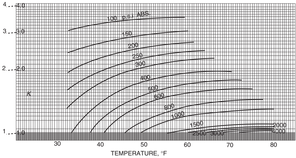
Figure 3.81 Vapor–solid equilibrium constant for methane (Carson & Katz, 1942, courtesy SPE-AIME).
