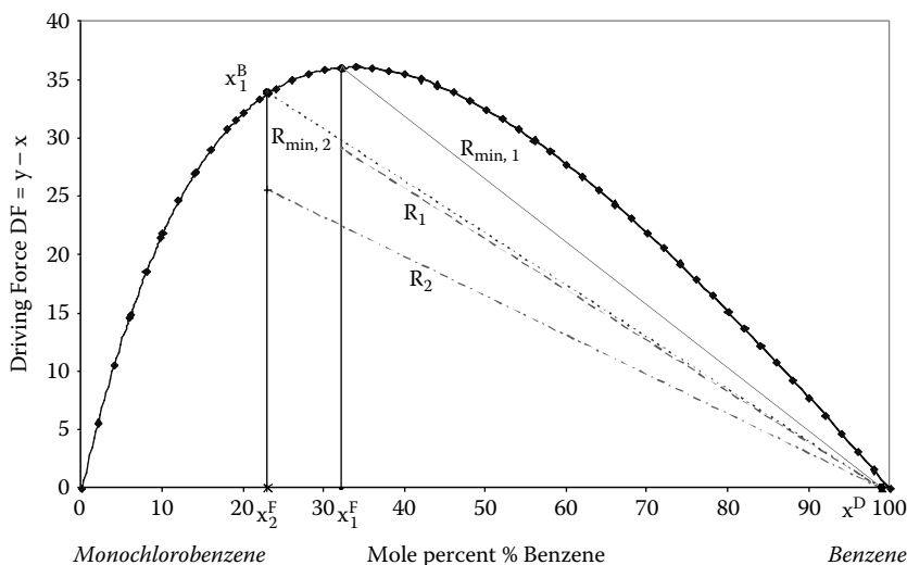
FIGURE 3.7 Driving force diagram for the binary system benzene–MCB.
