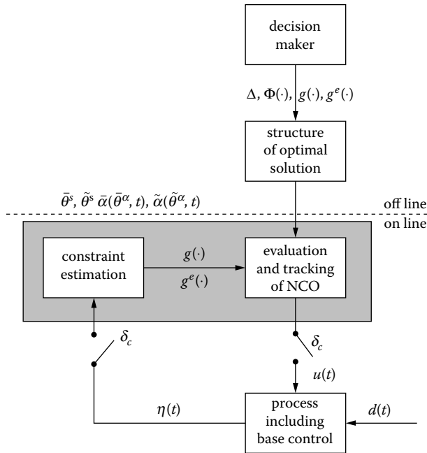
FIGURE 9.13 Tracking of necessary conditions of optimality.
