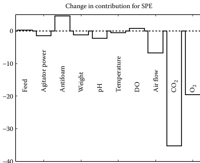
FIGURE 11.6 Contribution plot showing the change in the process from t = 67 to t = 73 . It is seen that the variables \text{CO}_2 and \text{O}_2 contribute most to the fault and that they are lower than normal. From the plot of the predicted final product concentration (Figure 11.5) it can be seen that the fault has a negative effect on the quality.
