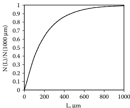
FIGURE 6.7 Normalized cumulative number distribution function.
