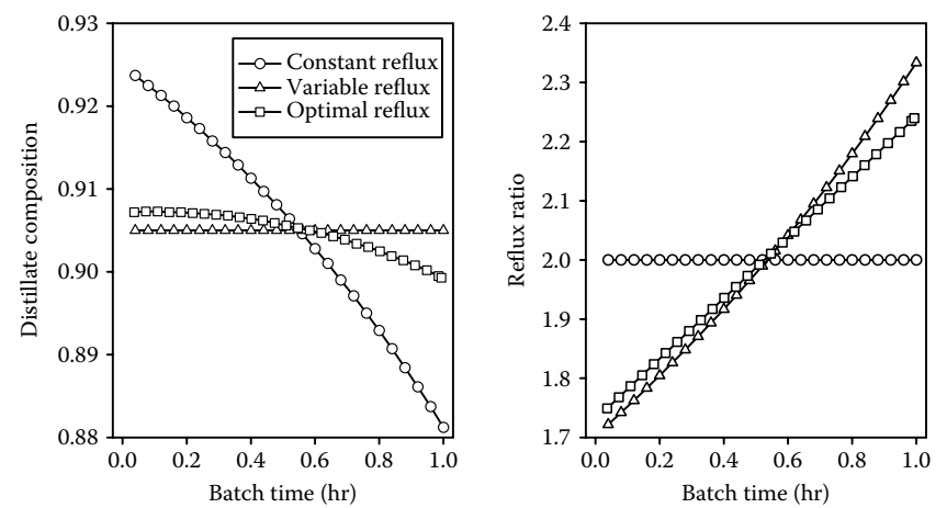
FIGURE 5.5 Three operating modes of batch rectification column.
