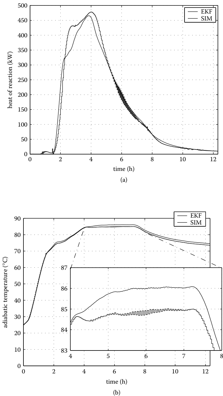
FIGURE 9.17 Online optimization: (top) estimation and prediction error of heat of reaction, and (bottom) adiabatic temperature.
