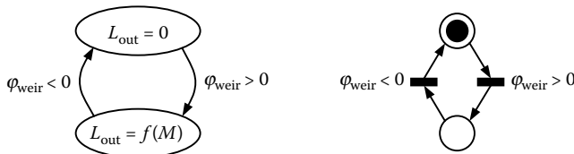
FIGURE 9.6 State graph (left) and Petri net (right) representation of tray hydraulics.
