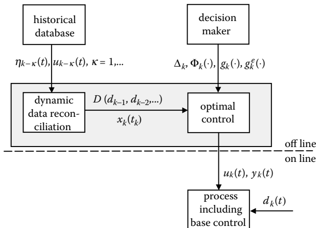
FIGURE 9.11 Batch-to-batch optimization.
