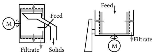
FIGURE 7.15 (Left) Peeler centrifuge and (right) vertical basket centrifuge. (From Friedmann, T., in Institute of Food Science: Laboratory of Food Process Engineering , ETH Zürich, Zürich, 1999. With permission.)
