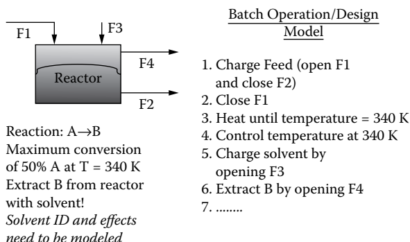
FIGURE 3.1 A solvent-based batch reaction process (process and operation models).
