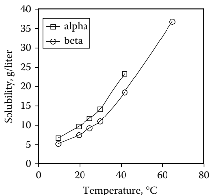
FIGURE 6.13 Solubility of \alpha and \beta forms of L-glutamic acid as a function of temperature. (From Kitamura, M., J. Crys. Growth , 96, 541–546, 1989 and Kitamura, M., J. Crys. Growth , 237–239, 2205–2214, 2004. With permission.)
