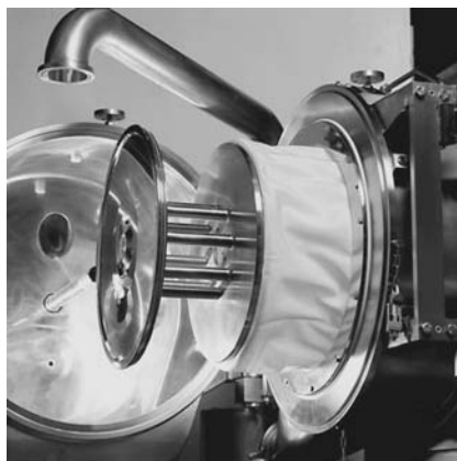
FIGURE 7.17 Open bowl of HF inverting filter centrifuge. (Image courtesy of HEINKEL AG.)
